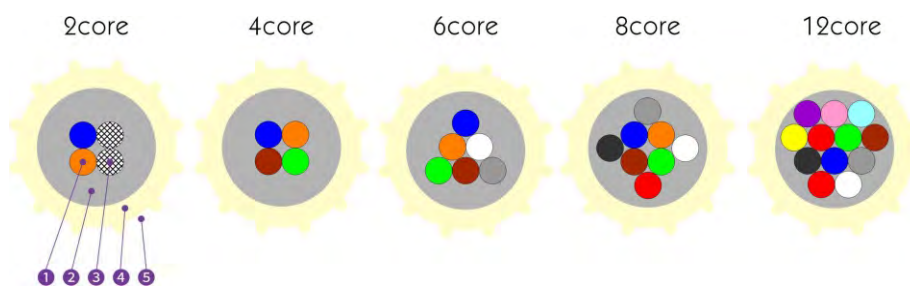
1,Optical Fibre 2,Resin 3,+2"Filled" Fibres 4, Low Friction Sheath 5, Groove
