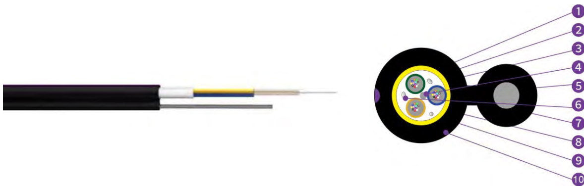
1, Fibre 2, Stripe 3, Loose Tube 4, FRP 5, Tube Filling Compound 6, Water Blocking Yarn 7, Steel Wire 8, APL 9, PE Sheath 10, Ripcord
